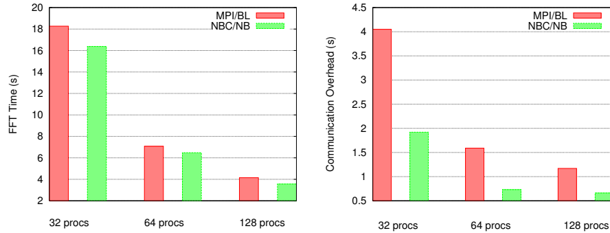
Fig. 3. Left: Blocking and non-blocking FFT times for different process counts on the XT4 system. Right: Communication overhead.
